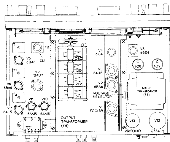
Plan view of Receiver
